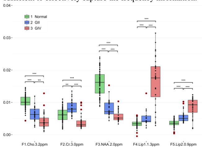
Figure 2: Boxplot of the five selected features among three tissue types (Normal: green; GII: blue; GIV: red). Red circled dots are the outliers of each group (***) indicates p < 0.0001 and ** indicates p < 0.001 .
