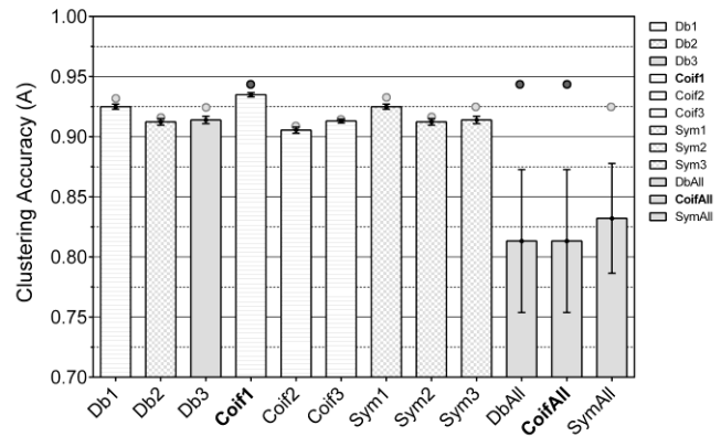
Figure 3: Comparison between different wavelet basis functions in terms of the obtained clustering accuracy ( A ) for both whole-spectral and sub-spectral analysis. Error bars represent the standard error of the mean (SEM). For the whole-spectral analysis, SEM was calculated with respect to different decomposition levels. For the sub-spectral analysis, SEM was computed with respect to various window sizes. Circles above the error bars indicate the maximum accuracy achieved by different wavelet basis functions.
